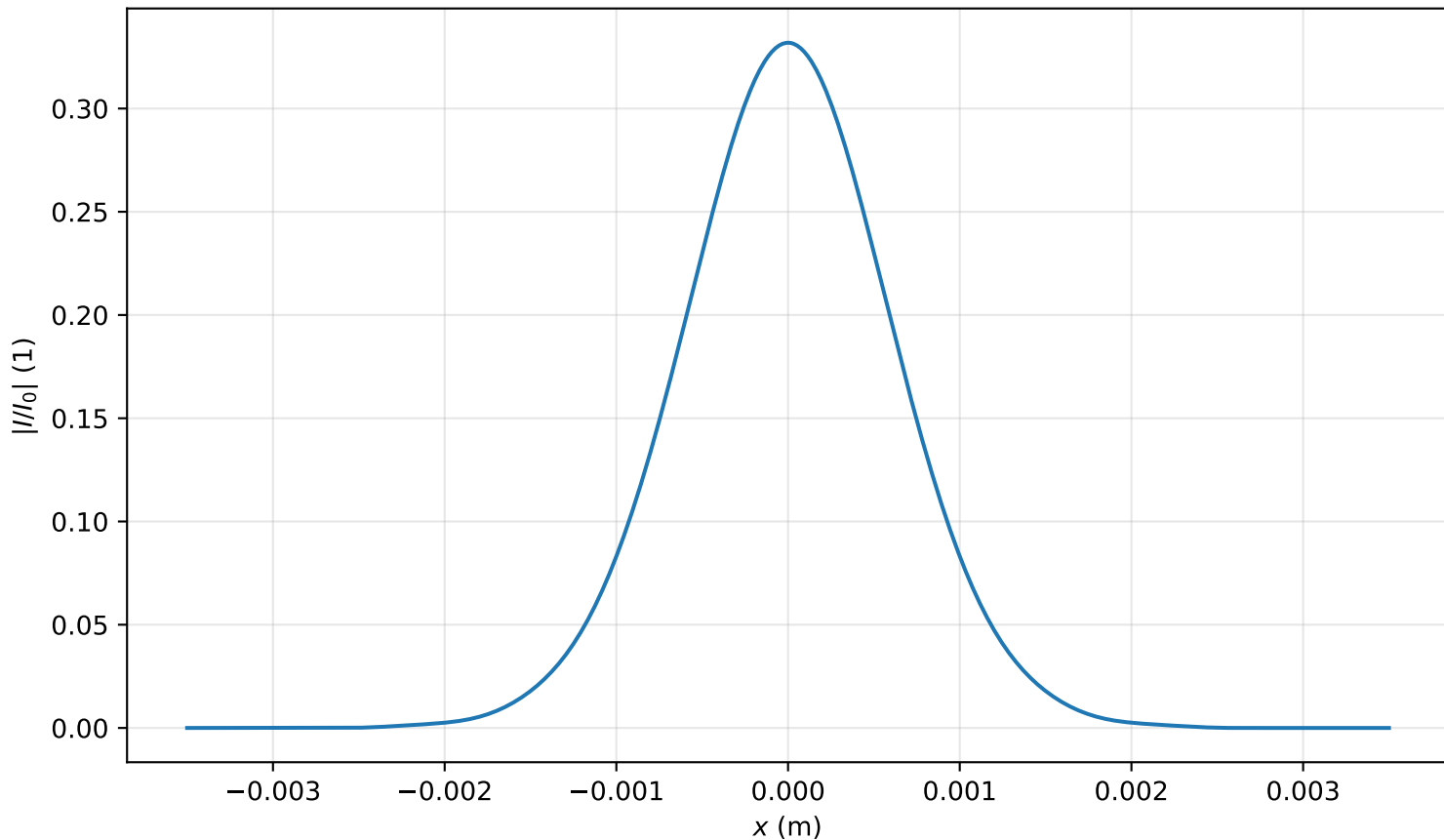
Intensity profile I(x, y = 0, z = 3.582m)/I_0 , P_{in}=0.3P_{cr} , artificial time
